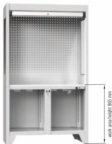
Quality station housing width 1200 mm
