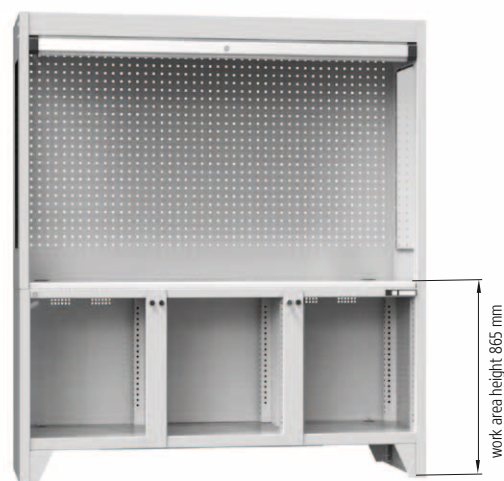
Quality station housing width 1800 mm
