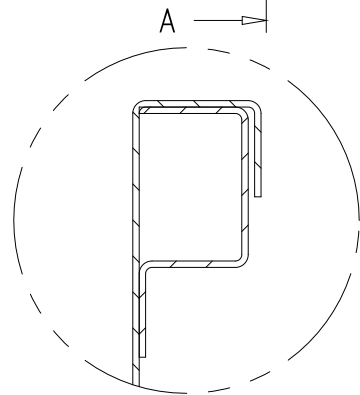
DETAIL B
